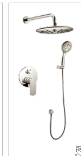
13717 01NPT Pressure balance valve (Φ40 cartridge)
